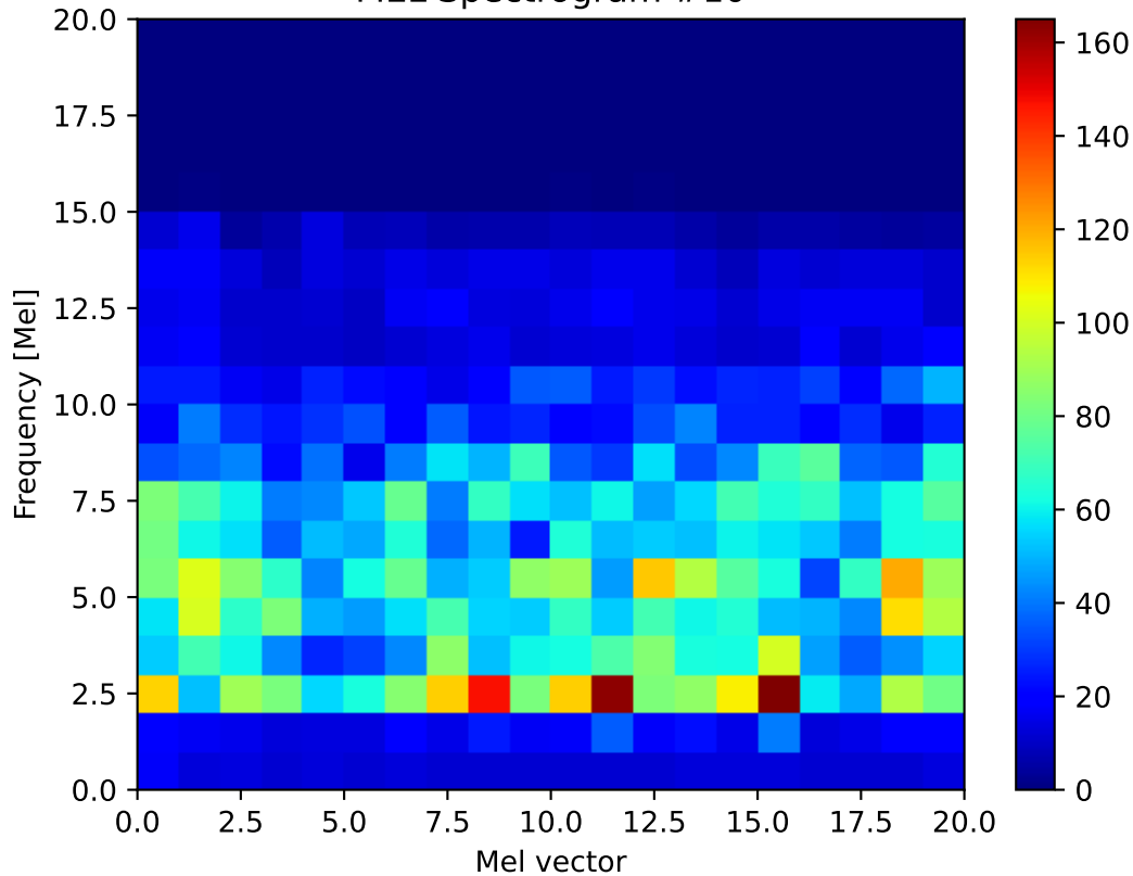
MEL Spectrogram #10
